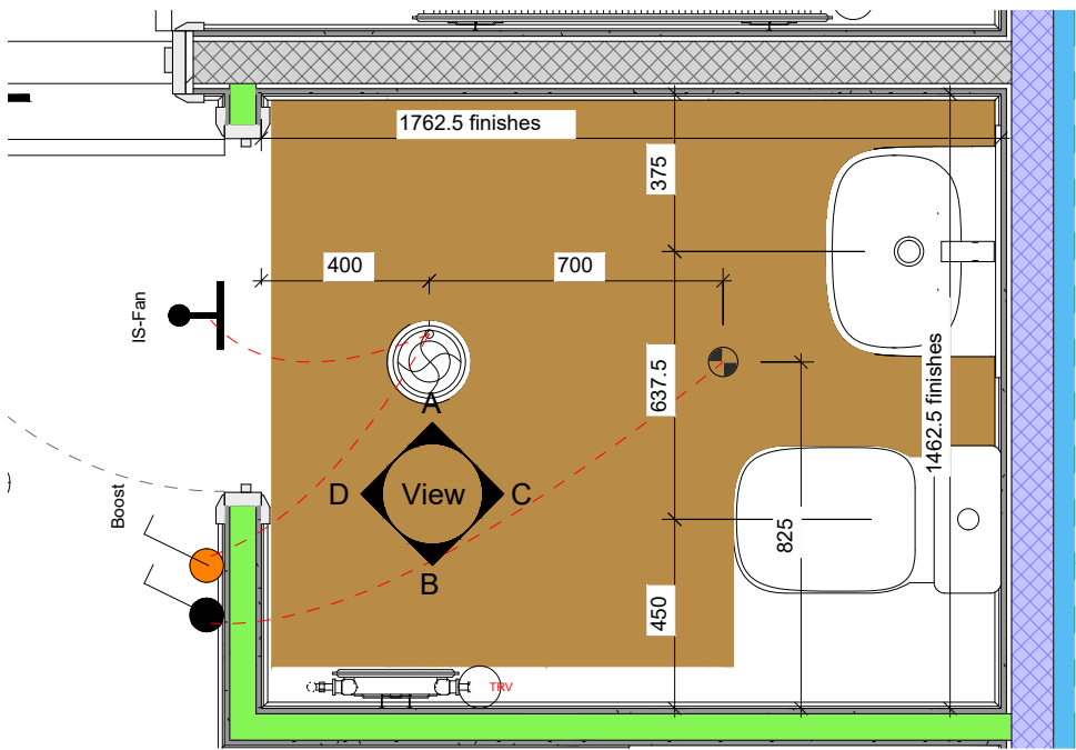
1 Ground Floor W/C Layout 1 : 20
