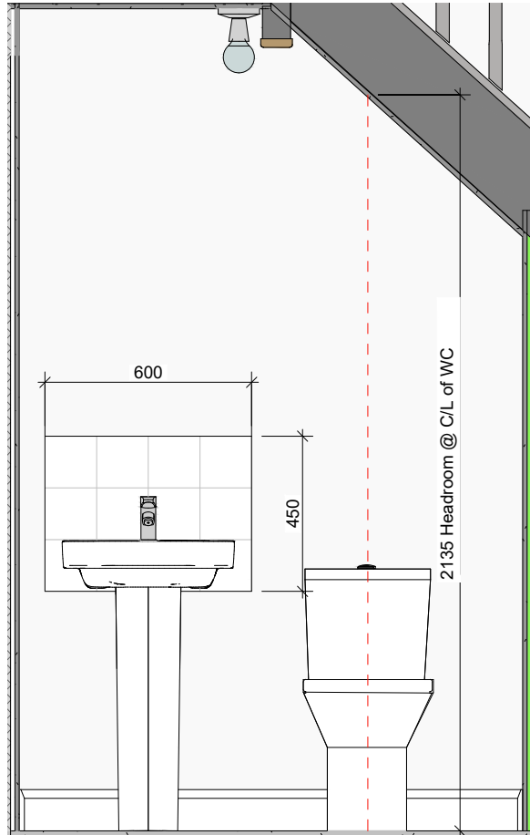
C WC - View C 1 : 20
